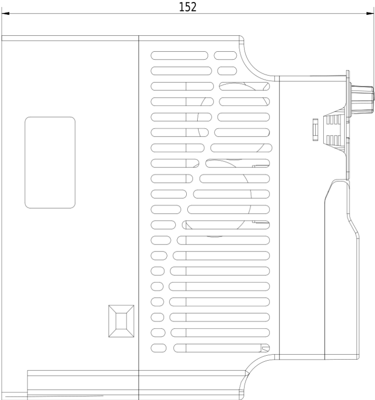
Dimensional drawing V800 - 1,5kW 4T0015
