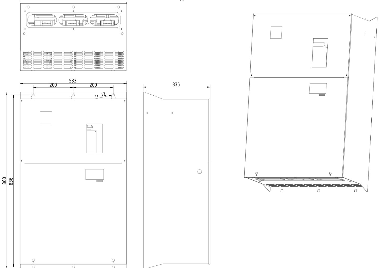
Dimensional drawing V810 - 200kW 4T2000
